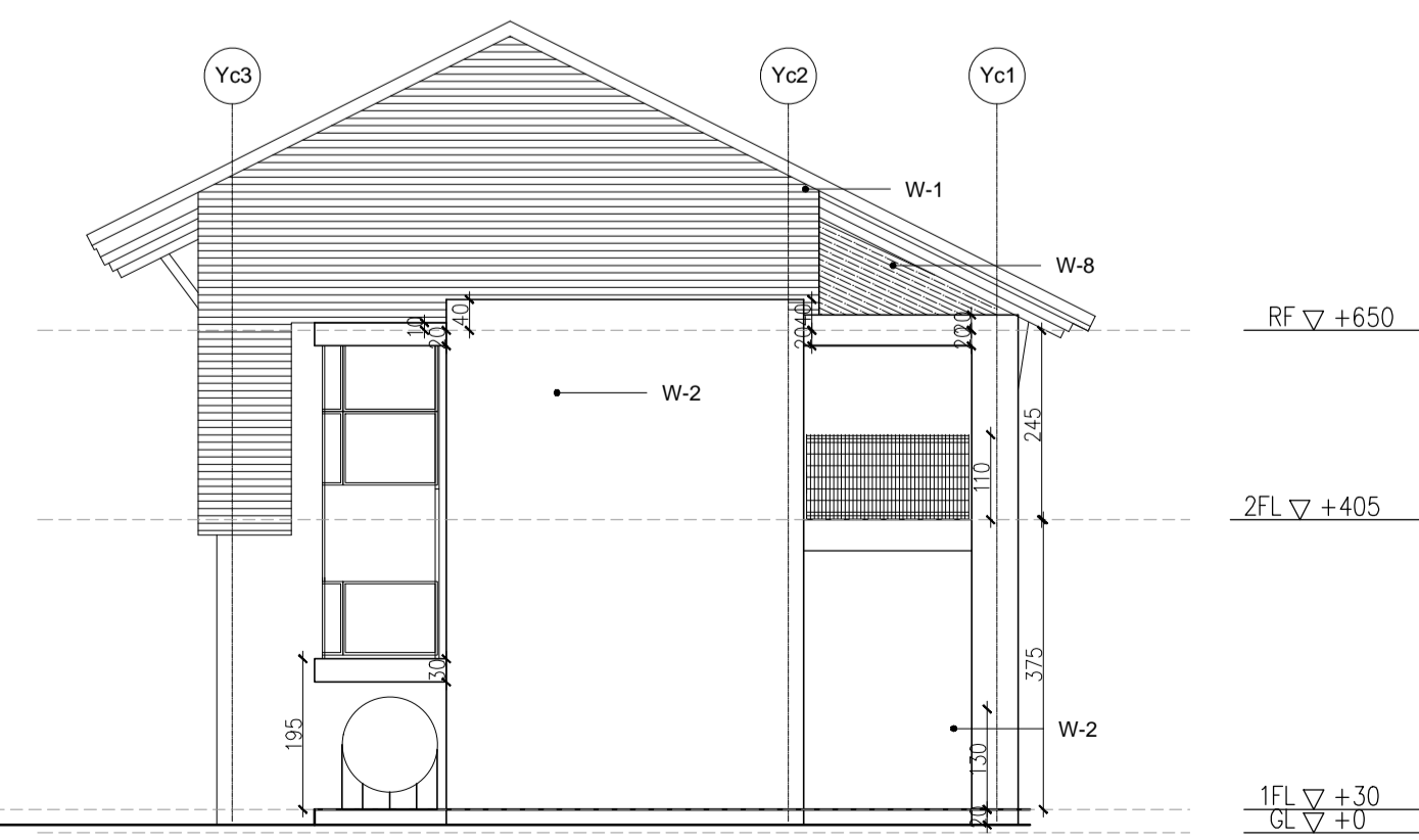
C棟西向立面圖 C Building West Elevation
